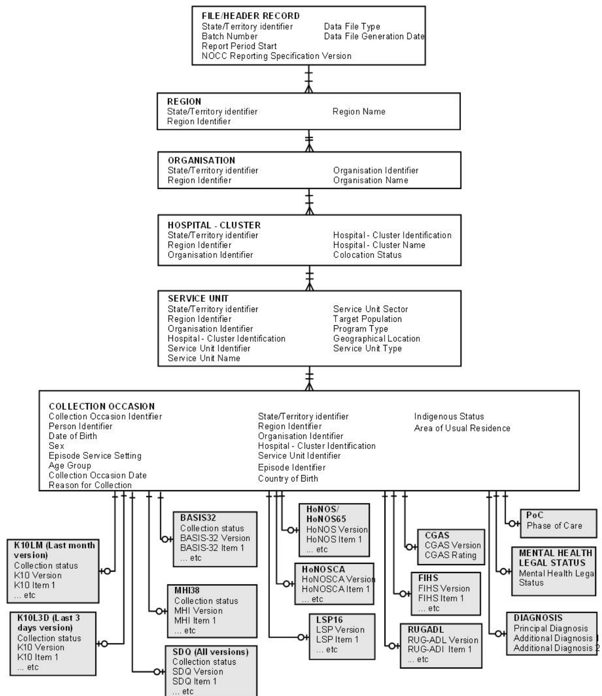
Figure 3: Data model underlying the NOCC data extract
